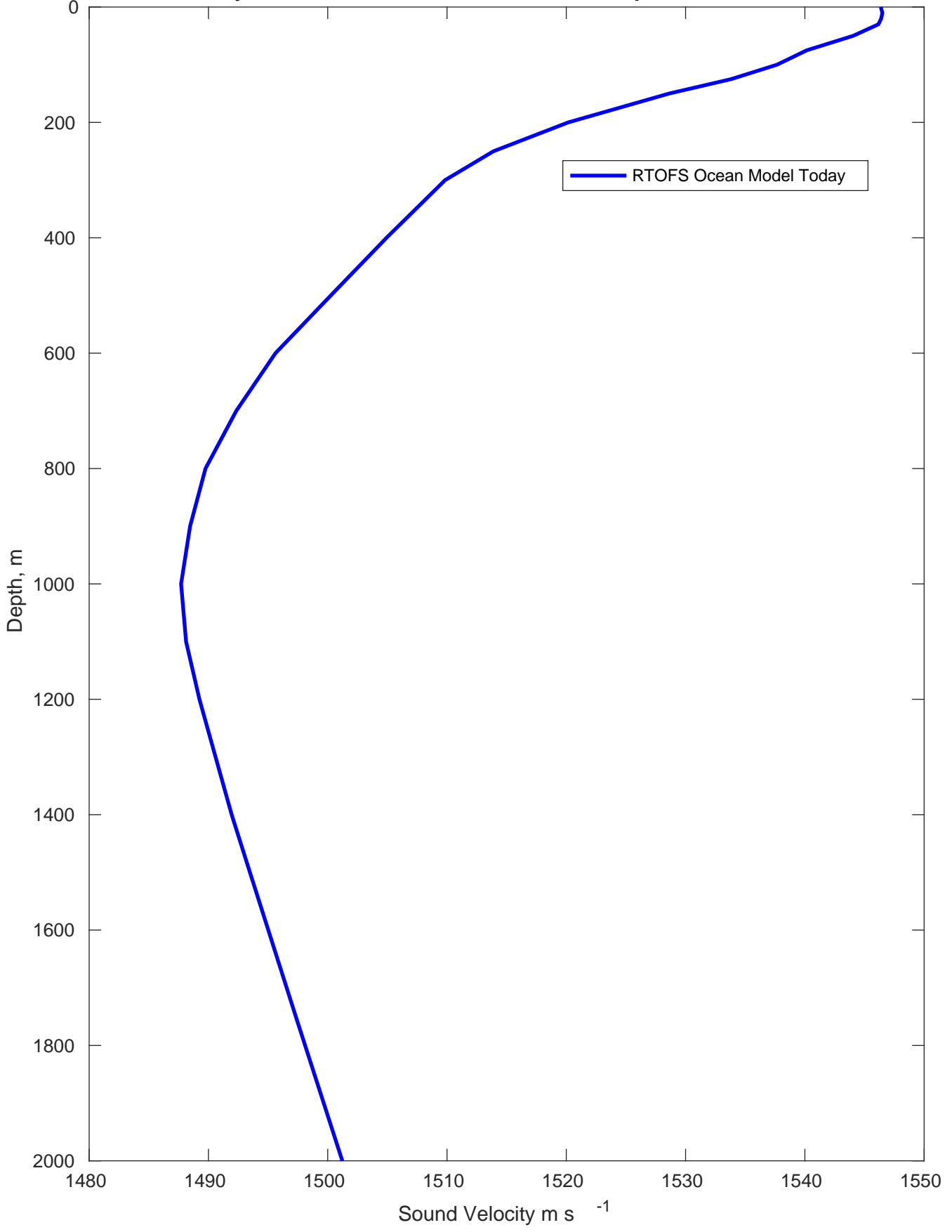
Sound Velocity Profile for BHP-WEL Trion GT on 03-Sep-2022 00:00:00
